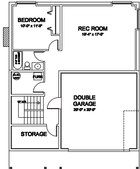
BASEMENT & FOUNDATION PLAN Floor Area = 885 SQ FT + Garage = 441 SQ FT
