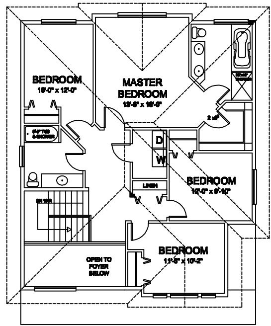
UPPER FLOOR PLAN Floor Area = 1139 SQ FT
